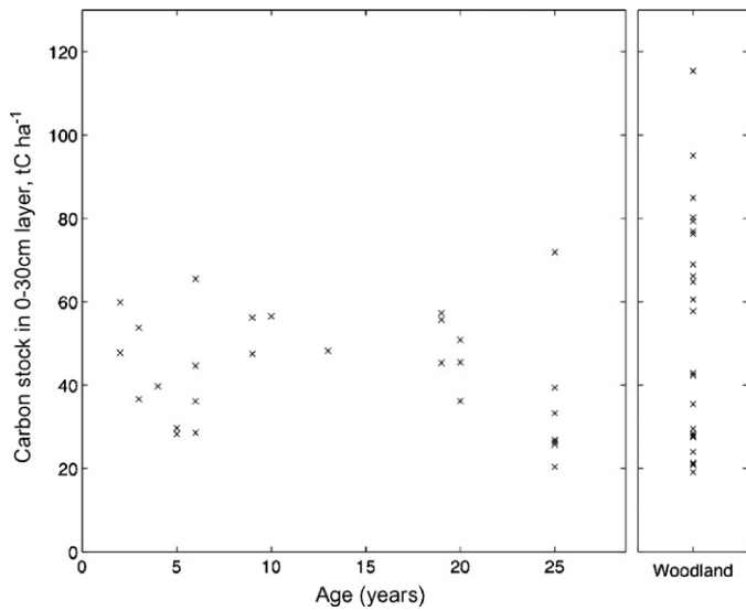
Fig. 6. Total soil C content in surface 0.3 m for all sites plotted against age for all abandoned machambas (left panel) and for woodlands (right panel). The age of the oldest abandoned machambas is given as 25 years, but lies between 20 and 30 years.
