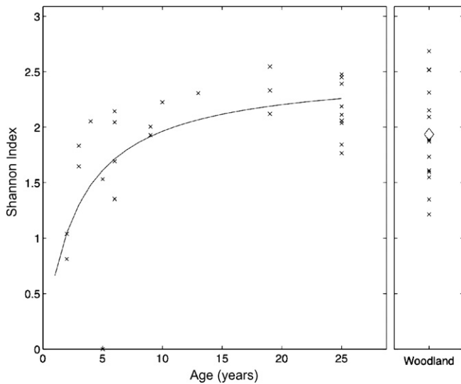
Fig. 5. Shannon index ( H' ) of species diversity plotted against age for all abandoned machambas (left panel), and for woodland plots (right panel, diamond indicates mean). The age of the oldest abandoned machambas is given as 25 years, but lies between 20 and 30 years. A non-linear curve fit for the chronosequence of abandoned machambas is shown, using a saturation equation, H' = \alpha t / (\beta + t) , where t is the time since abandonment (years) and \alpha and \beta are the parameters. For the best fit \alpha = 2.51 and \beta = 2.79 .
