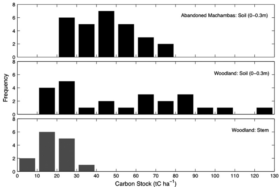
Fig. 7. Frequency distributions of C stocks ( \text{t C ha}^{-1} ) in abandoned machamba soils (top panel), woodland soils (middle) and woodland stem C (bottom panel).
